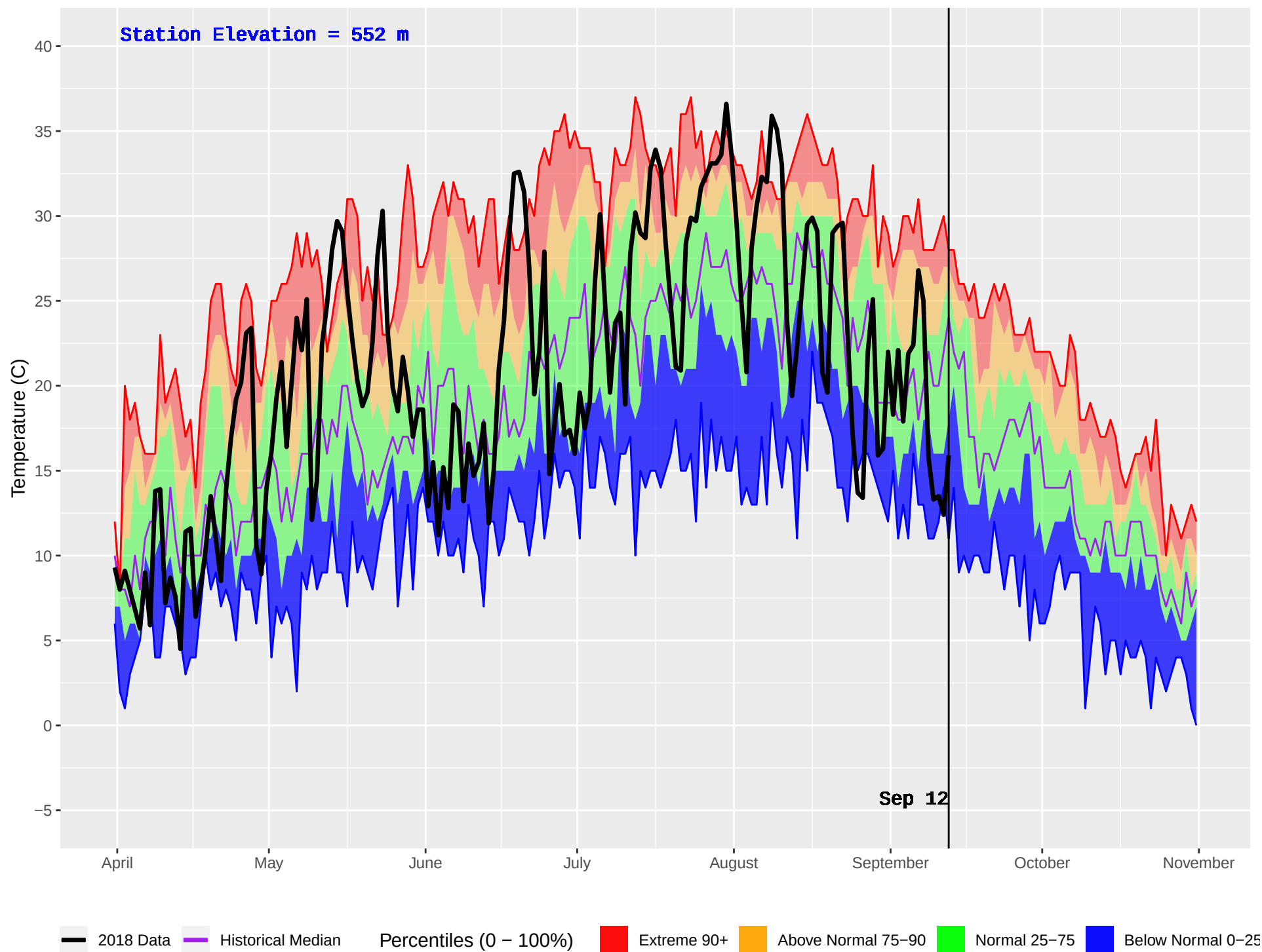
NAHATLATCH (316) : Historical (2001–2016) and Current (2018) Daily Temperature
