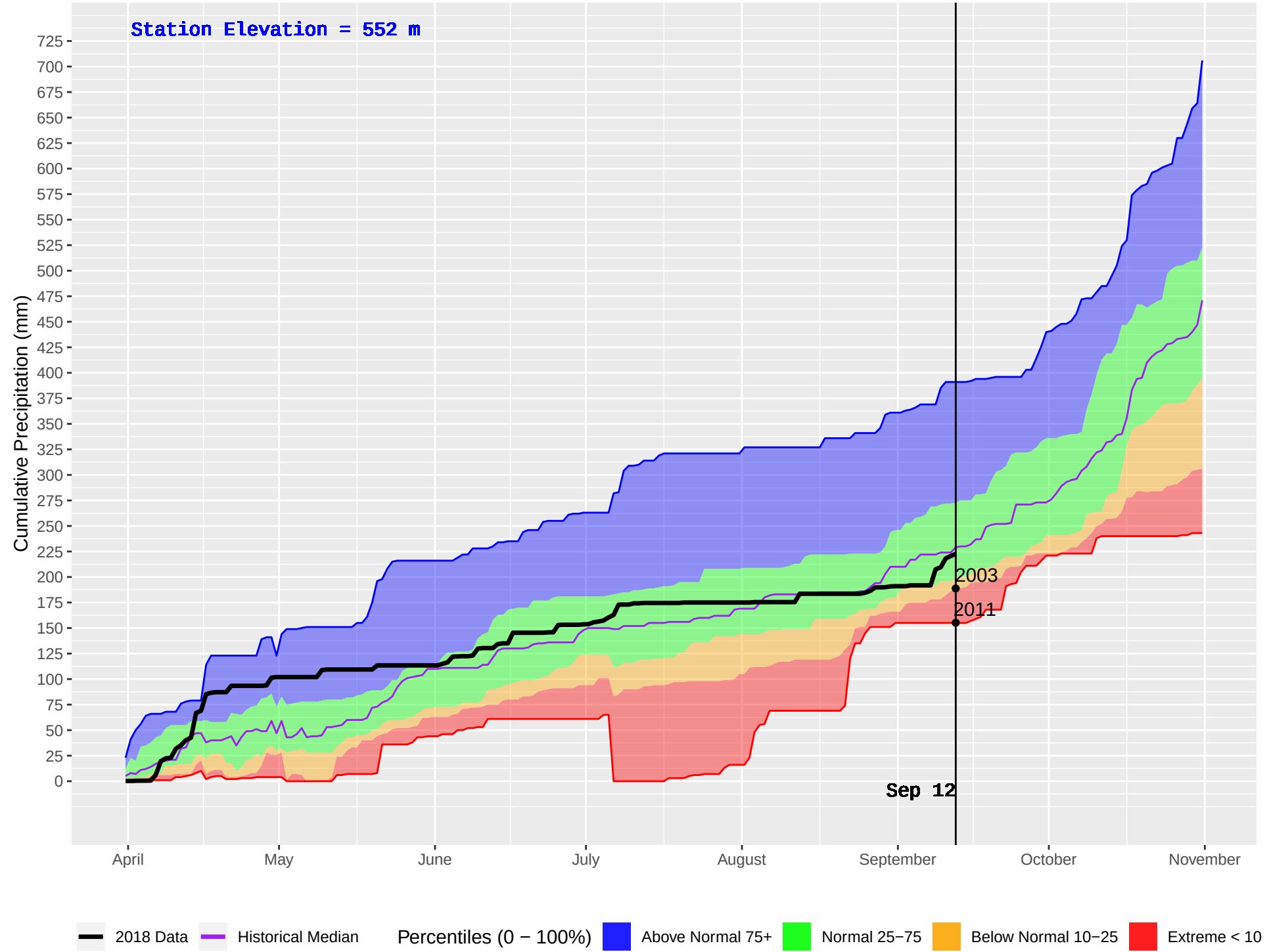
NAHATLATCH (316) : Historical (2001–2016) and Current (2018) Daily Cumulative Precipitation
