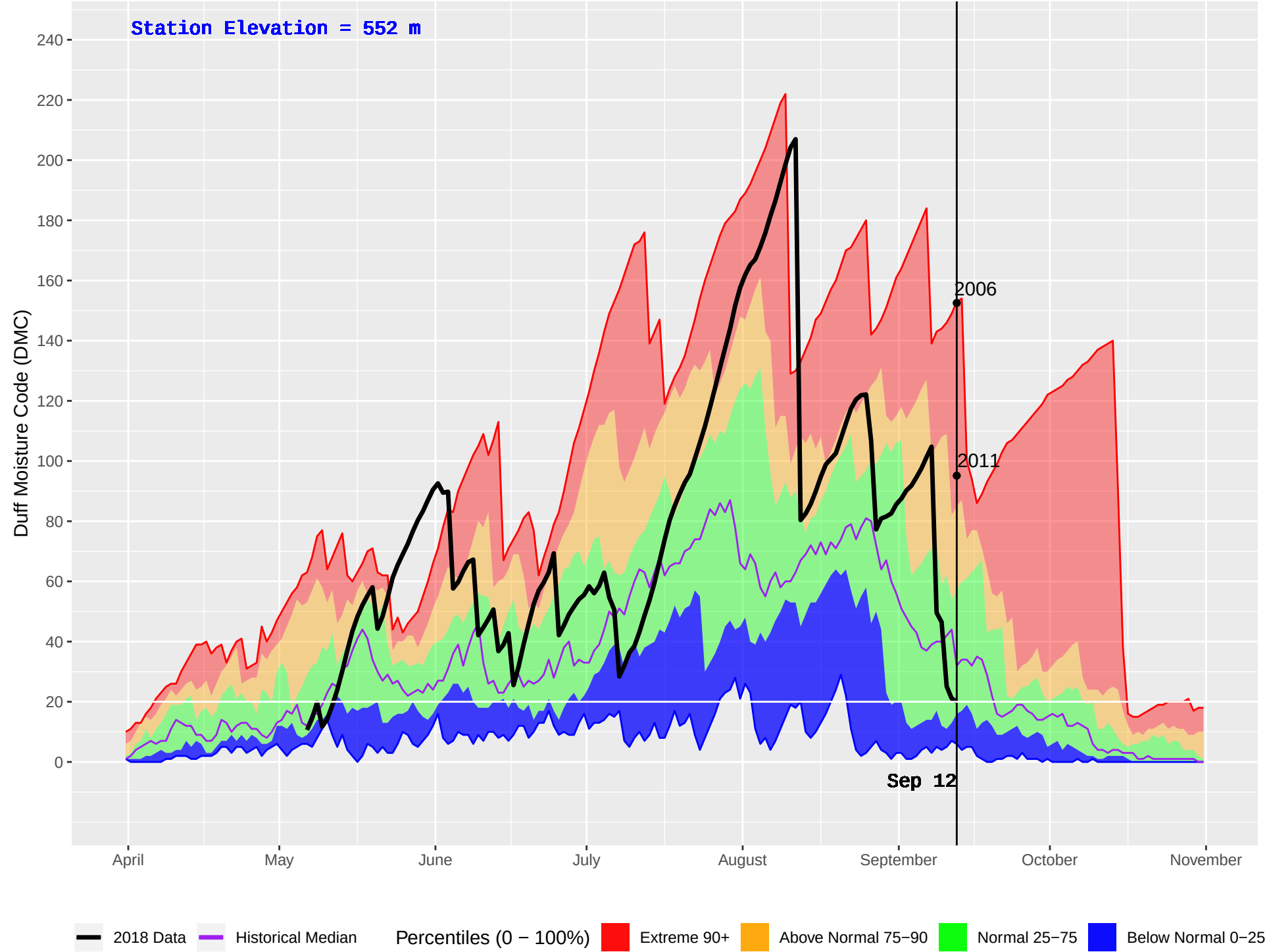
NAHATLATCH (316) : Historical (2001–2016) and Current (2018) Daily Duff Moisture Code (DMC)
