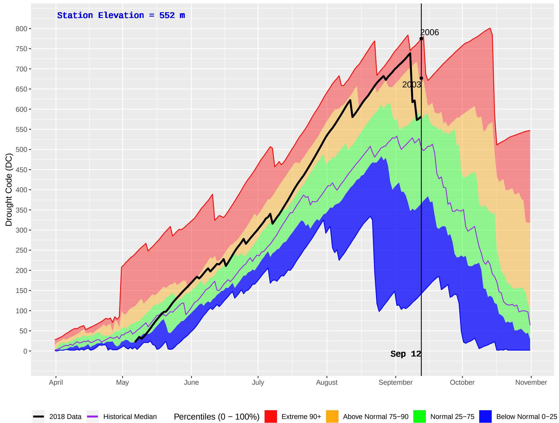
NAHATLATCH (316) : Historical (2001–2016) and Current (2018) Daily Drought Code (DC)
