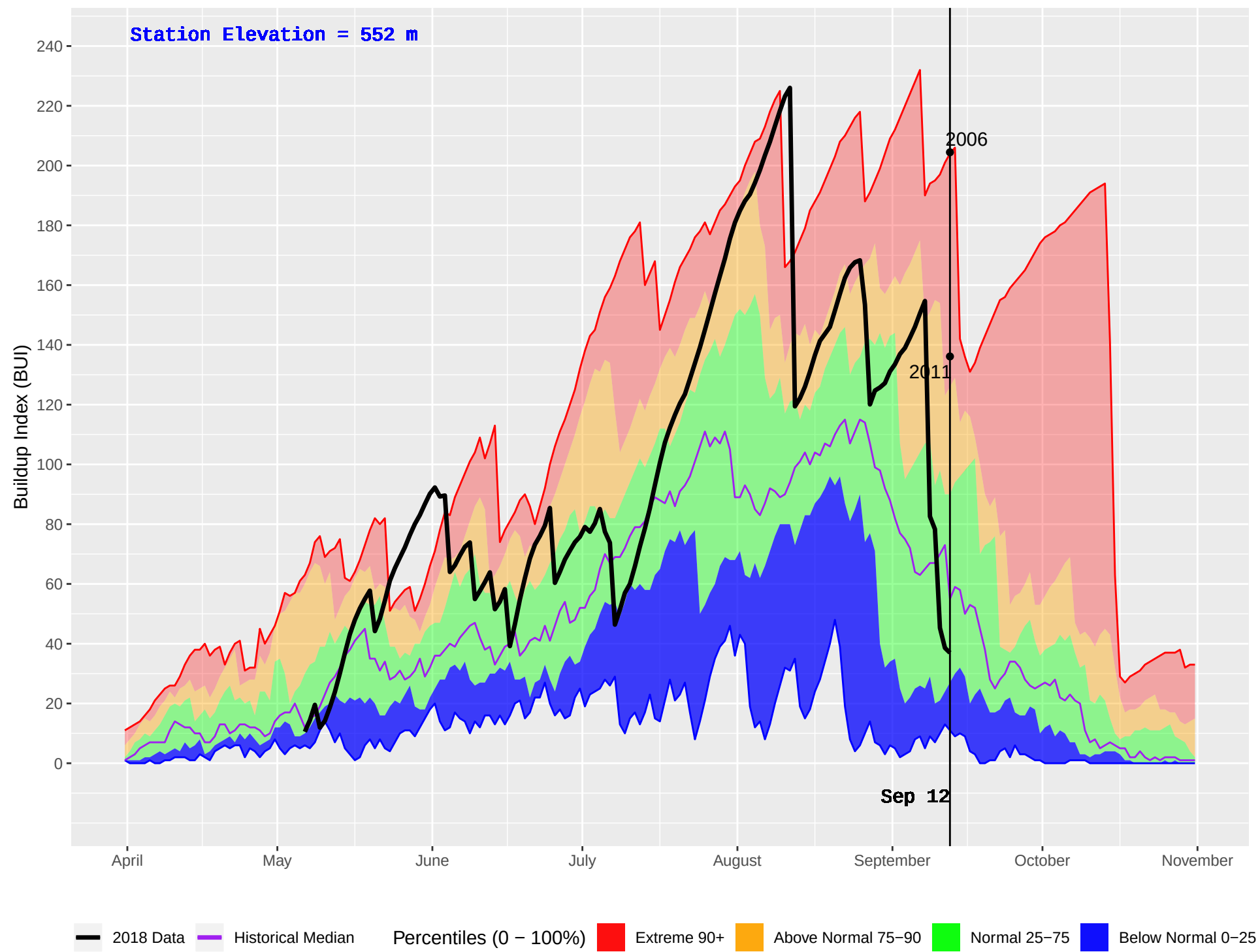
NAHATLATCH (316) : Historical (2001–2016) and Current (2018) Daily Buildup Index (BUI)
