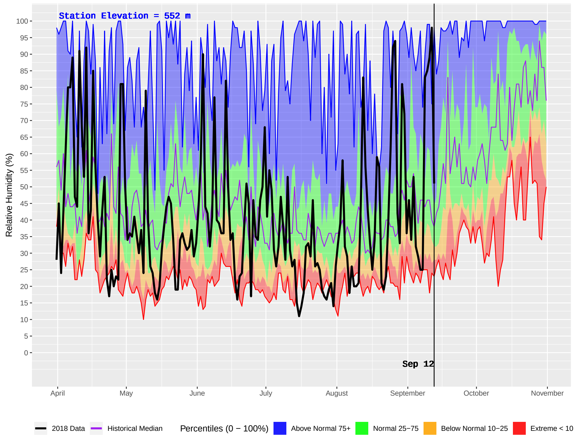
NAHATLATCH (316) : Historical (2001–2016) and Current (2018) Daily Relative Humidity
